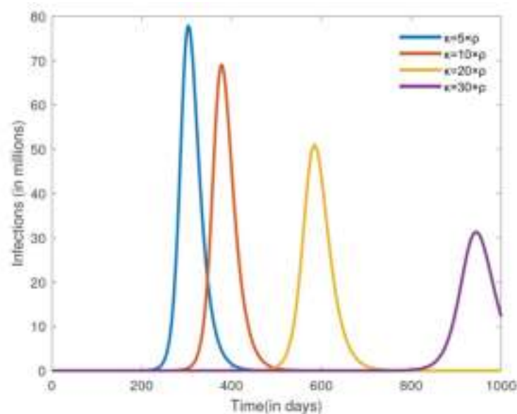
Figure 6. Numerical simulation of the number of infections for different misinformed recovery rates \kappa . The other parameter values are fixed at \Lambda = 0 , \alpha = 0.25 \times 10^{-4} , \beta = 1/14 , \rho = 0.1 , \sigma = 0.5 \times 10^{-3} , \gamma = 10^{-4} , \theta = 4 \times 10^{-5} , \mu_0 = 0.0025 , and \mu_1 = 0.01 .
