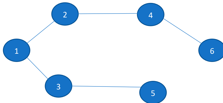
Figure 3. Index-restricted SCN of the network in Table 1.
