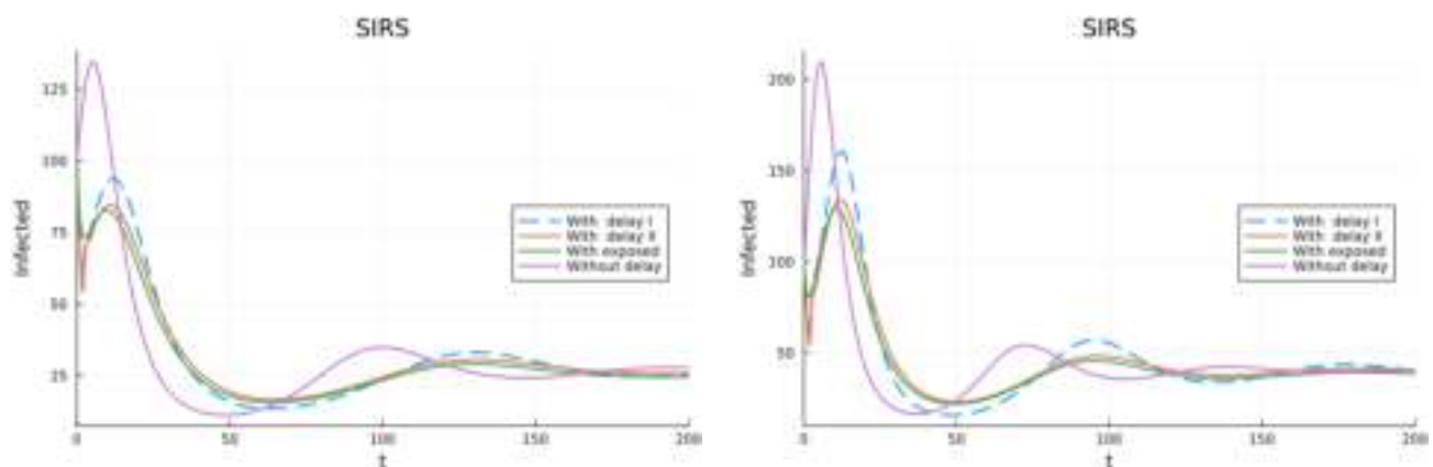
Figure 8. Model with two populations with total temporal immunity leaving the R compartment at different rates. (left) \beta = 0.5 . (right) \beta = 0.666
