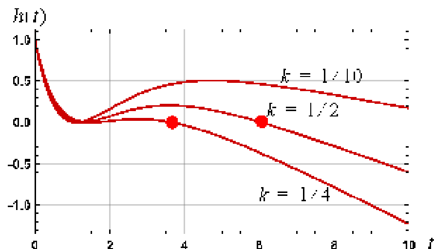
Figure 11. Graph of the impulse response of the transfer function defined by (69) for values of k \in \{1/10, 1/4, 1/2\} .
