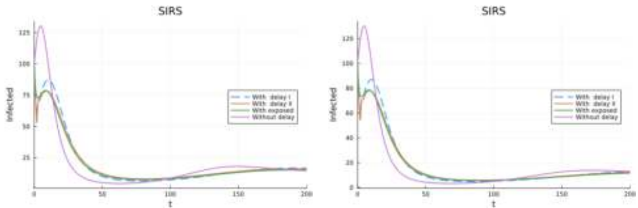
Figure 14. Model with recovered getting partial permanent immunity and vaccinated getting total immunity that in one case wanes and in the other does not. (left) Vaccination immunity wanes. (right) Vaccination immunity does not wane.
