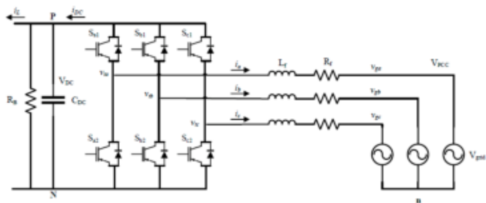
Figure 10. Two-level VSC with an L filter and a DC link circuit bleed resistor.
