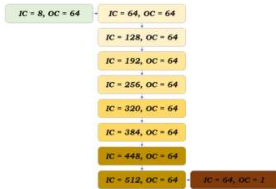
Figure 1. The model architecture. Each rectangle represents a layer, and the two numbers indicate the number of input and the number of output channels. In each layer, there are two convolutional operations as in Equation (1). In the intermediate layers, each output is concatenated to the input of the same layer and is passed to the next layer.
