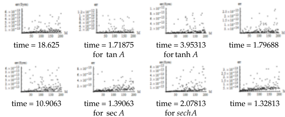
Figure 4. Error of the \tan A , \sec A , \tanh A , and \operatorname{sech} A for two algorithms.
