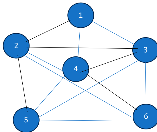
Figure 4. Given G(6, 13) network.
