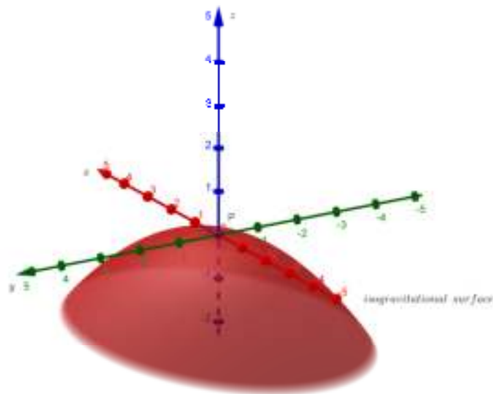
Figure 1. Isogravitational Surface.
