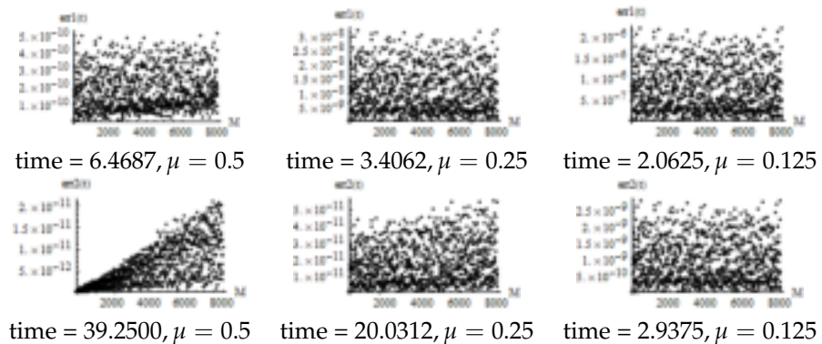
Figure 8. Error of numerical solution (8) for several algorithms.
