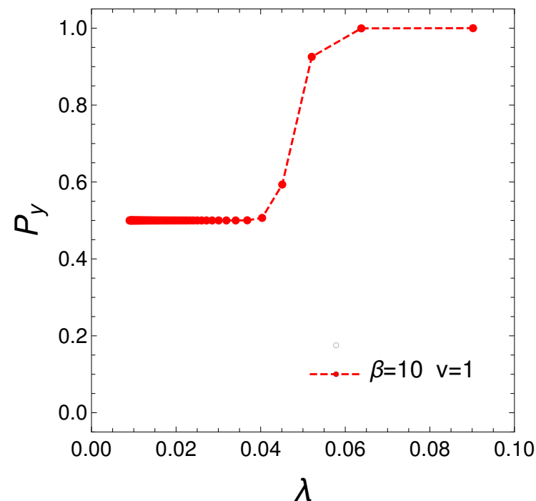
Figure 2. Purity versus de Broglie thermal wavelength (in meters) for \beta = 10 , N = 20 , and v = 1 . When the purity is small, the wavelength is also small, and vice versa when the purity approaches unity. One detects a minimum purity equal to one-half (see text).
