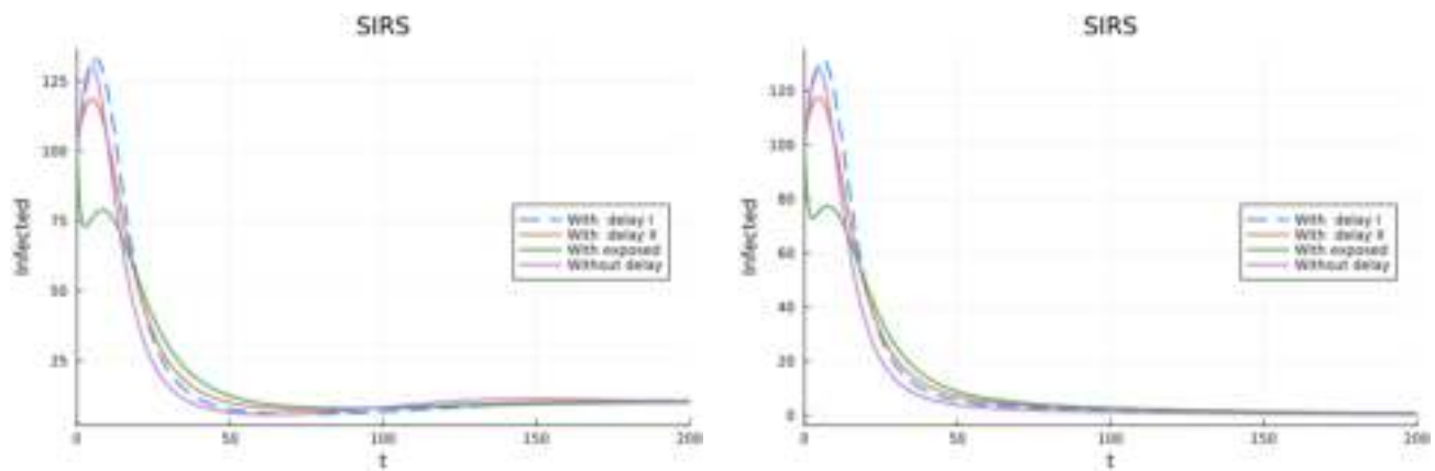
Figure 15. Model with two classes of vaccinated individuals, one with total and permanent immunity and the other with total immunity that wanes to partial and permanent immunity. (left) Waning vaccination immunity. (right) Permanent vaccination immunity.
