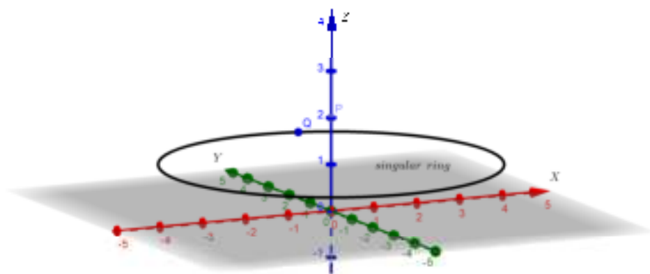
Figure 2. Singular Ring.
