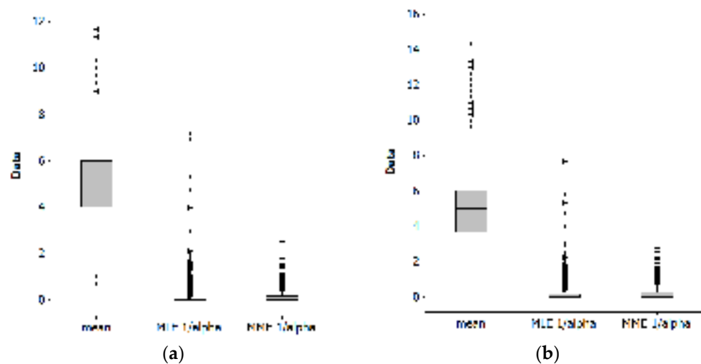
Figure 2. Monte Carlo simulation experiment boxplots (as usual, asterisks denote outliers). Left (a): NB2[5, 5(1 + 5/0.0476)]. Right (b): NB2[5, 5(1 + 5/0.1600)].
