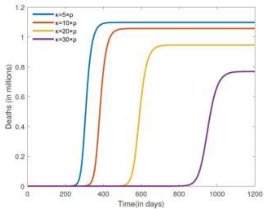
Figure 7. Numerical simulation cumulative deaths for different recovery rates \kappa . The other parameter values are fixed at \Lambda = 0 , \alpha = 0.25 \times 10^{-4} , \beta = 1/14 , \rho = 0.1 , \sigma = 0.5 \times 10^{-3} , \gamma = 10^{-4} , \theta = 4 \times 10^{-5} , \mu_0 = 0.0025 , and \mu_1 = 0.01 .
