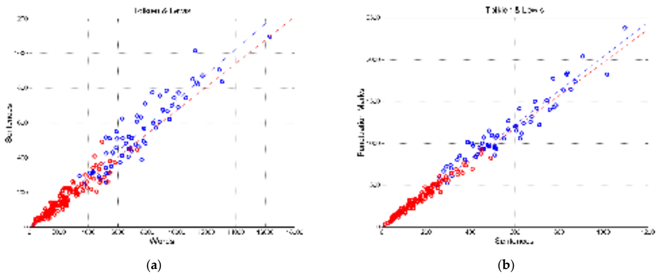
Figure 7. (a) Scatterplot of n_S versus n_W in Lord (blue) and Trilogy (red); (b) n_I versus n_S in Lord (blue) and Trilogy (red).
