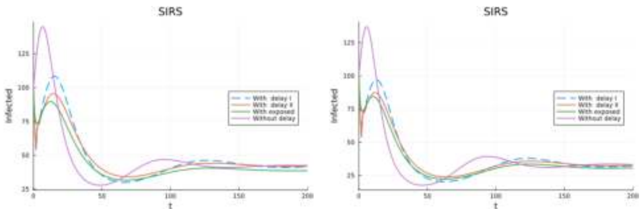
Figure 10. Simulations for the model with two classes, one with total and immunity, and the other with partial immunity, both temporal. (left) \beta_p = \beta/2 . (right) \beta_p = \beta/8 .
