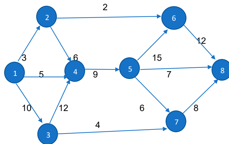
Figure 9. Directed network.
