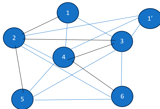
Figure 5. Modified network G(7, 16) .
