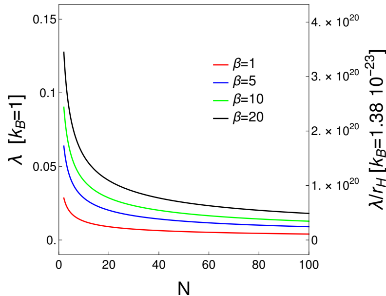
Figure 1. Thermal length quantifier \lambda vs. N for several values of \beta = 1, 5, 10 , and 20 (in meters for the left vertical scale and in terms of the Hydrogen atom radius in the right vertical scale) taking k_B = 1 (left) and k_B = 1.380648 \times 10^{-23} (right). We see that the thermal length decreases as the number of fermions in the system grows, at rates regulated by the temperature. The rates increase as the temperature decreases. The length becomes smaller as N grows, which can be read as a vestige of classicality. That the effects are more noticeable for lower temperatures than for higher ones, is something that one should intuitively expect.
