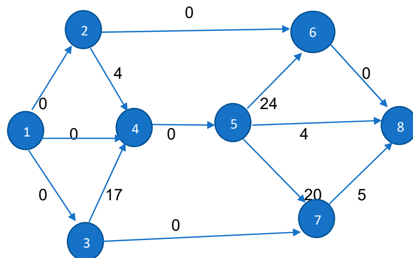
Figure 10. The final reconstructed network after 7 iterations.
