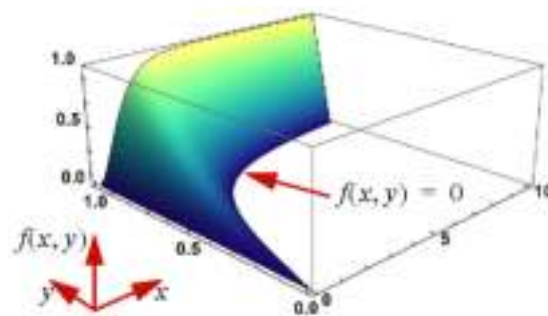
Figure 2. Graph of f(x, y) .
