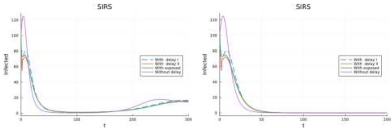
Figure 13. Model with vaccination. Infected individuals get total immunity that wanes to partial and permanent immunity. Vaccinated individuals get total immunity that may wane or not. (left) Vaccination immunity wanes to partial permanent. (right) Vaccination immunity does not wane.
