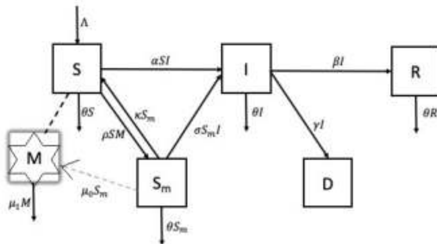
Figure 1. Schematic diagram of COVID-19 transmission with misinformation. Individuals transition from compartments S and S_m to compartment I as a result of their interaction with individuals in compartment I . Individuals transition between compartments S and S_m as a result of interaction with misinform M (either by consuming it or recovering from it). Misinformation density is produced by individuals in compartment S_m .
