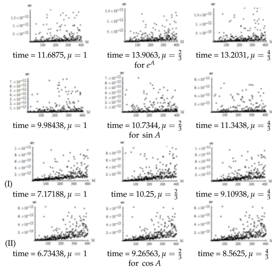
Figure 1. Error comparison of the algorithms in Table 1 for \mu = 1, \frac{2}{3}, \frac{4}{3} .
