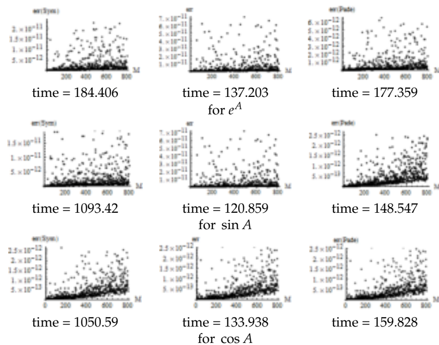
Figure 2. Error of e^A , \cos A , and \sin A for three algorithms.
