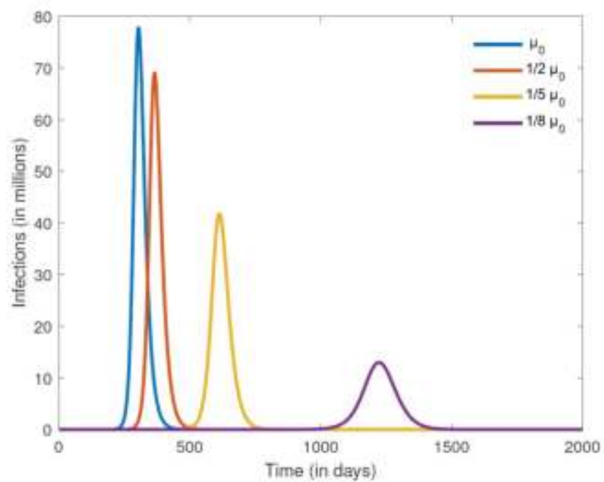
Figure 8. Numerical simulation of the number of infections for different misinformation growth rates \mu_0 . The other parameter values are fixed at \Lambda = 0 , \alpha = 0.25 \times 10^{-4} , \beta = 1/14 , \rho = 0.1 , \kappa = 5\rho , \sigma = 0.5 \times 10^{-3} , \gamma = 10^{-4} , \theta = 4 \times 10^{-5} , and \mu_1 = 0.01 .
