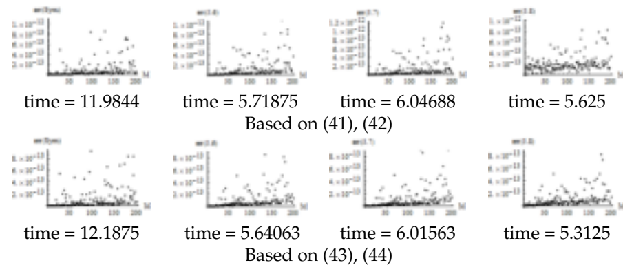
Figure 6. Error of \ln A for the several algorithms.
