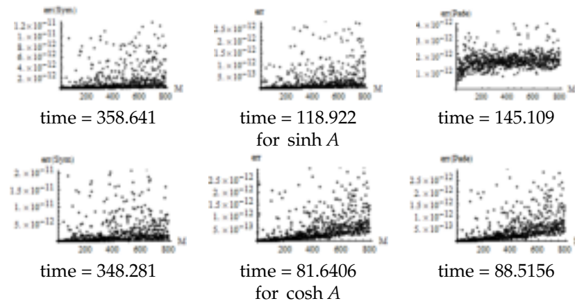
Figure 3. Error of \sinh A and \cosh A for three algorithms.
