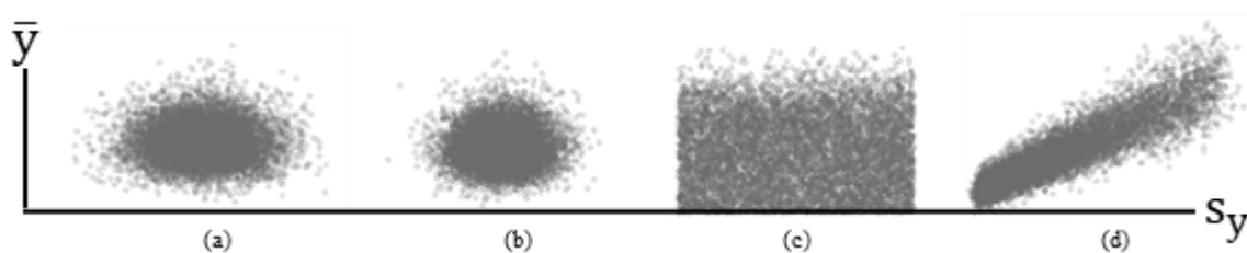
Figure 1. Selected simulated (10,000 replications, n = 100 ) relationships between \bar{y} and s^2 . Left (a): iid normal RVs. Left middle (b): iid NB2 RVs. Right middle (c): i~id normal RVs. Right (d): i~id NBp RVs.
