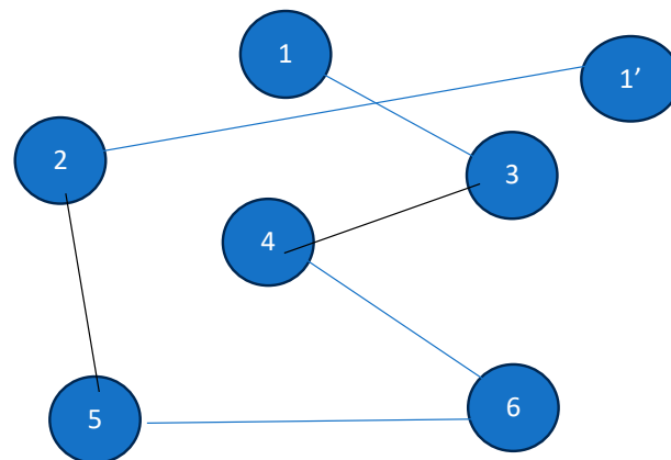
Figure 7. The path 1 -> 3 -> 4 -> 6 -> 5 -> 2 -> 1'.
