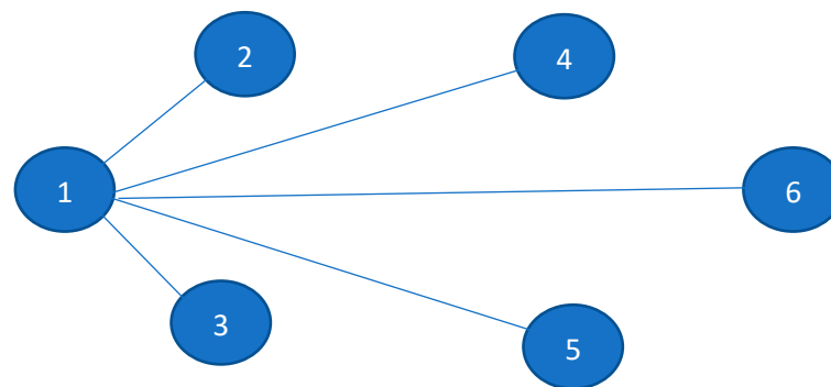
Figure 1. Shortest connected graph of the network from Table 1.
