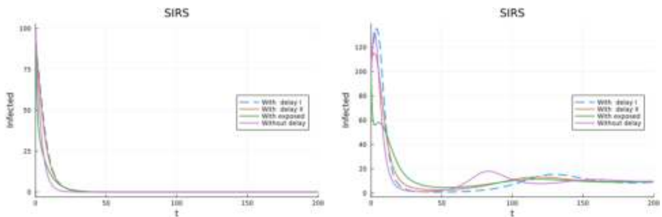
Figure 16. Model with vaccination, antivirals and isolation (30). (left) \beta = 0.5 . (right) \beta = 1 .
