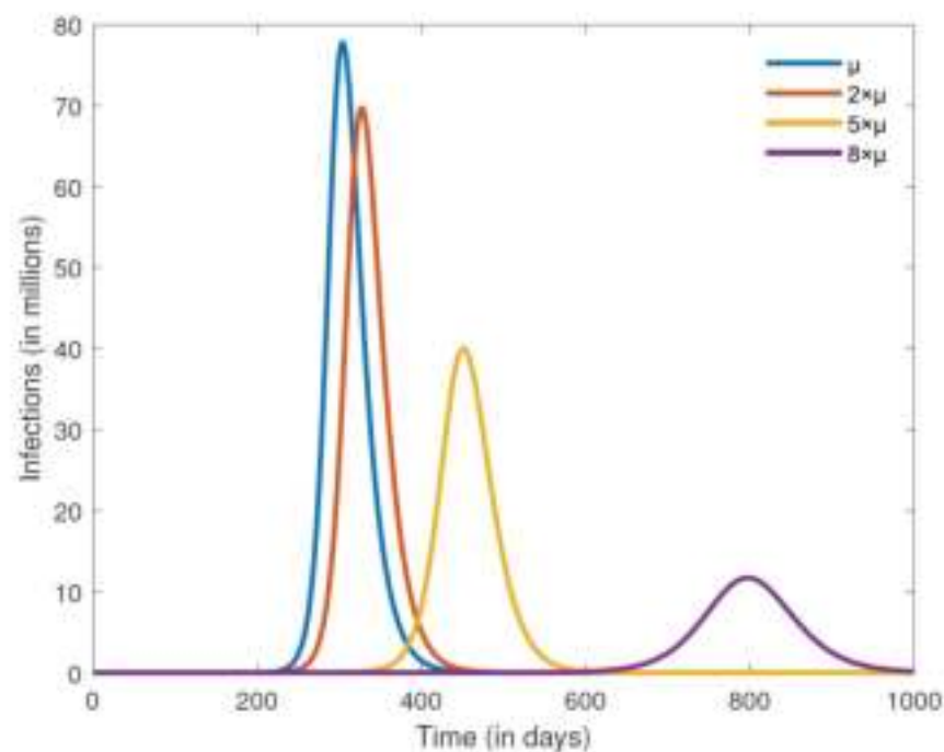
Figure 9. Numerical simulation of the number of infections for different misinformation decay rates \mu_1 = \mu . The other parameter values are fixed at \Lambda = 0 , \alpha = 0.25 \times 10^{-4} , \beta = 1/14 , \rho = 0.1 , \kappa = 5\rho , \sigma = 0.5 \times 10^{-3} , \gamma = 10^{-4} , \theta = 4 \times 10^{-5} , and \mu_0 = 0.0025 .
