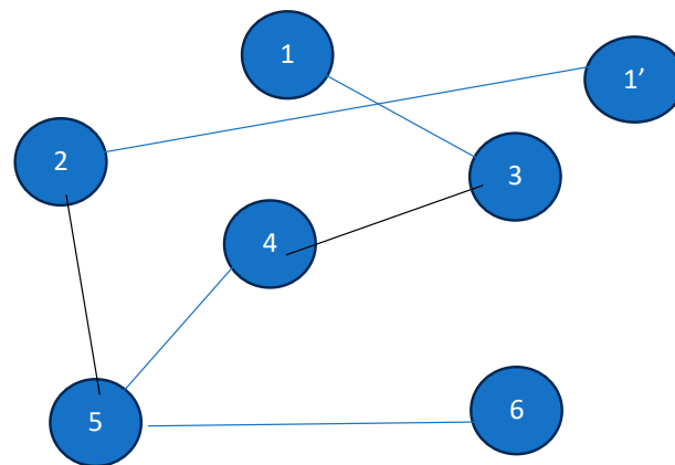
Figure 6. Spanning trees by greedy approach.
