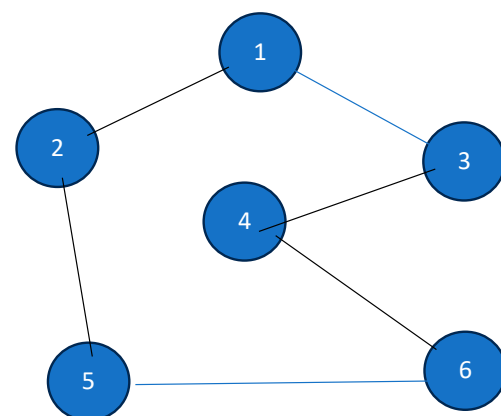
Figure 8. The spanning tree and the minimum travelling salesman tour.
