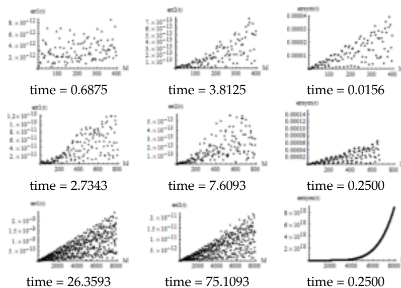
Figure 7. Error of numerical solution (8) for several algorithms ( nn is calculated according to (64)).
