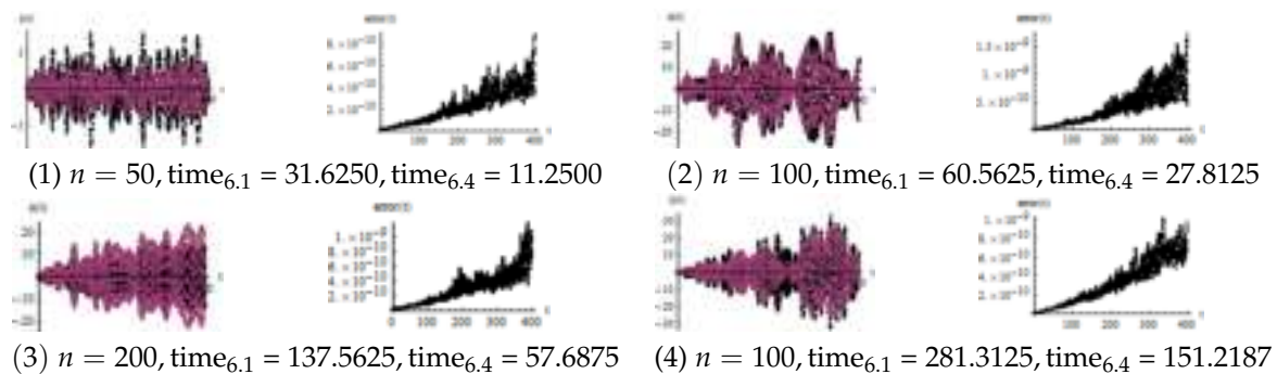
Figure 9. Numerical solutions and errors of two algorithms.
