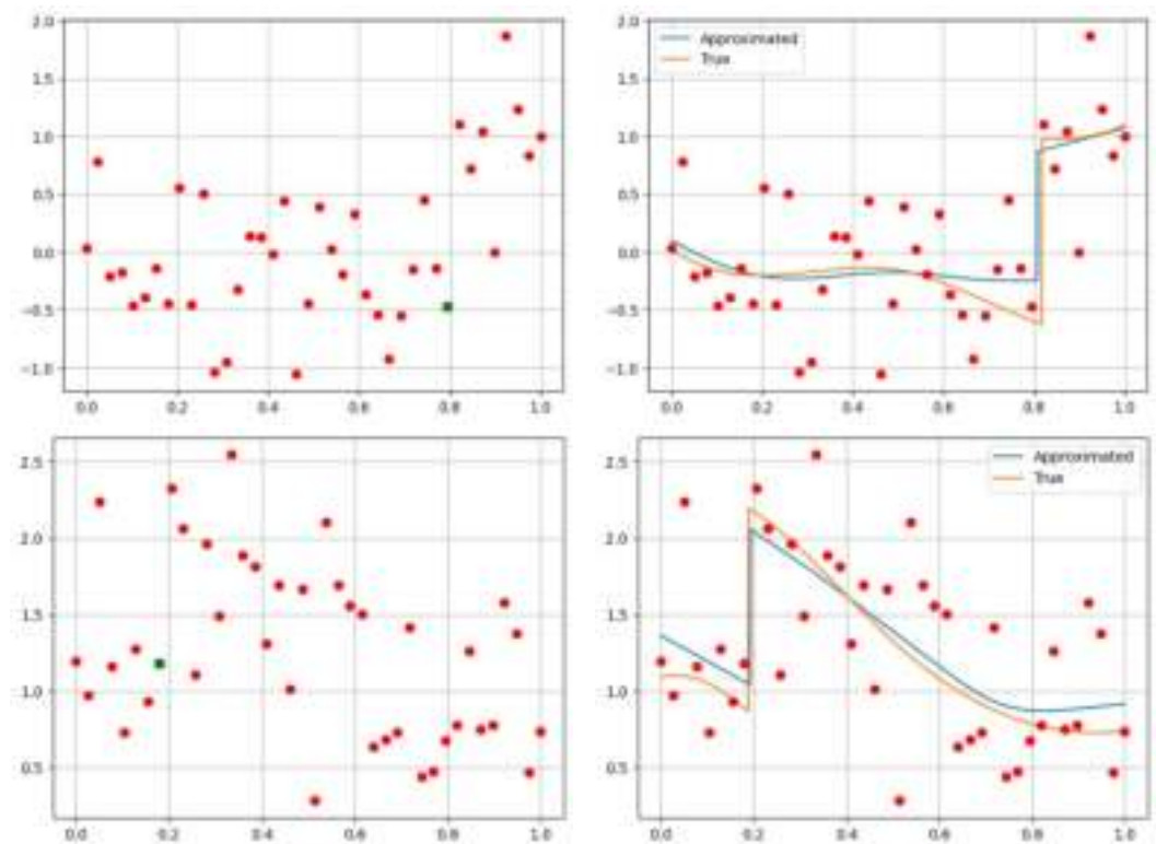
Figure 3. We demonstrate our method visually by approximating the location of the discontinuity point of two univariate piecewise smooth functions from their samples, to which white noise was added. The upper-left and lower-left figures show the samples with the added noise. All samples are red-colored except for the point that indicates the closest sample from the right to the jump discontinuity, which is green-colored. Our approach found the green point. The upper-right and the lower-right figures show the approximations for the two functions, which were achieved using two cubic splines for each one of the functions.
