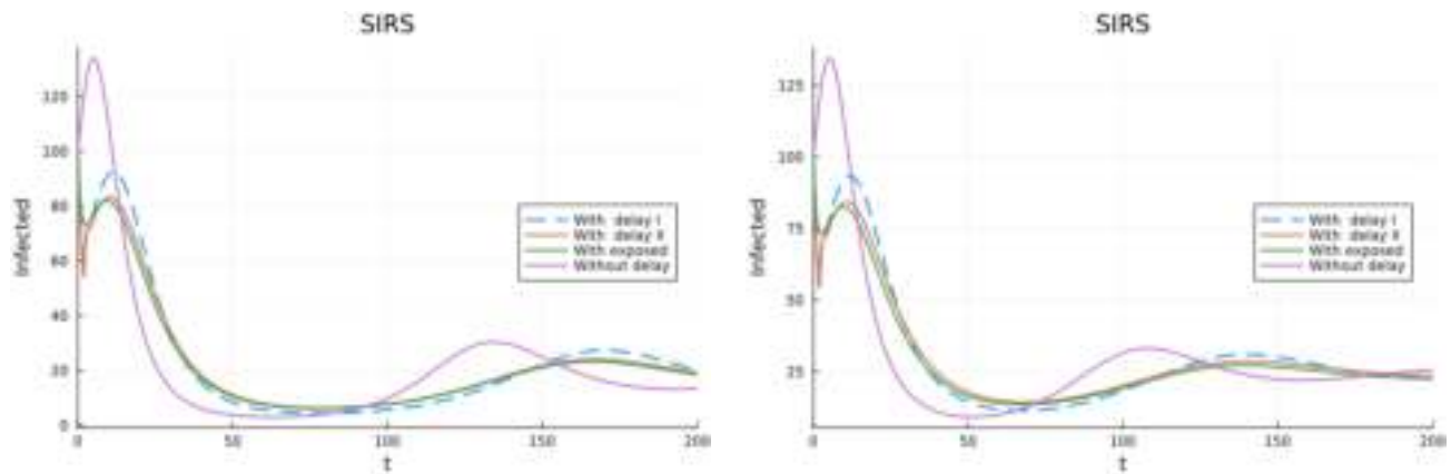
Figure 7. Model with total temporal and then partial temporal immunity (left) \beta_p = 0.25 . (right) \beta_p = 0.4 .
