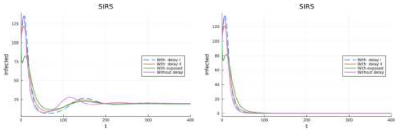
Figure 11. Model with two population classes. Both get total immunity (compartment R) and then lose it to get partial immunity at different rates with different infection rates. (left) \beta_1 = 0.9\beta, \beta_2 = 0.8\beta . (right) \beta_1 = 0.45\beta, \beta_2 = 0.4\beta .
