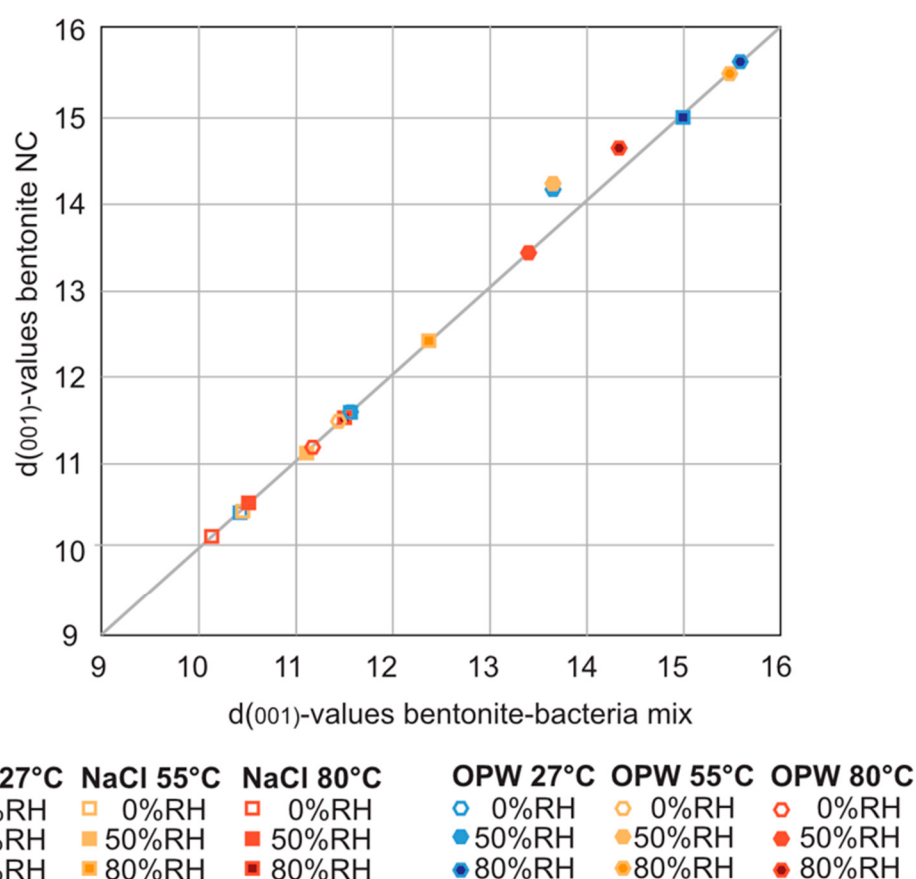
Figure 3. Correlation curve of d(001)-values of montmorillonite with (x-axis) and without bacteria (y-axis) in NaCl, and OPW solutions at different temperatures and humidities (see also Table S1).
